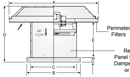
Model HRSB-F Filtered Belt Drive Model HRSD-F Filtered Direct Drive
