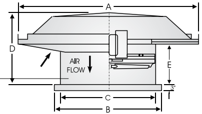
Model HRSB Supply Belt Drive Model HRSD Supply Direct Drive
