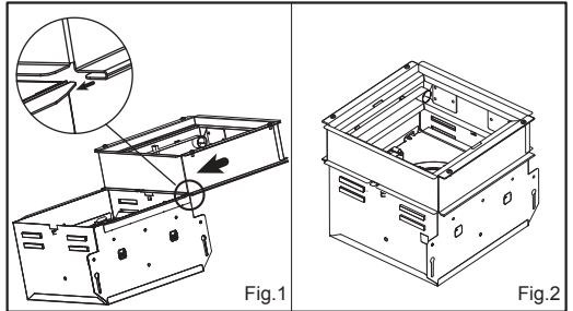
Damper Assembly
